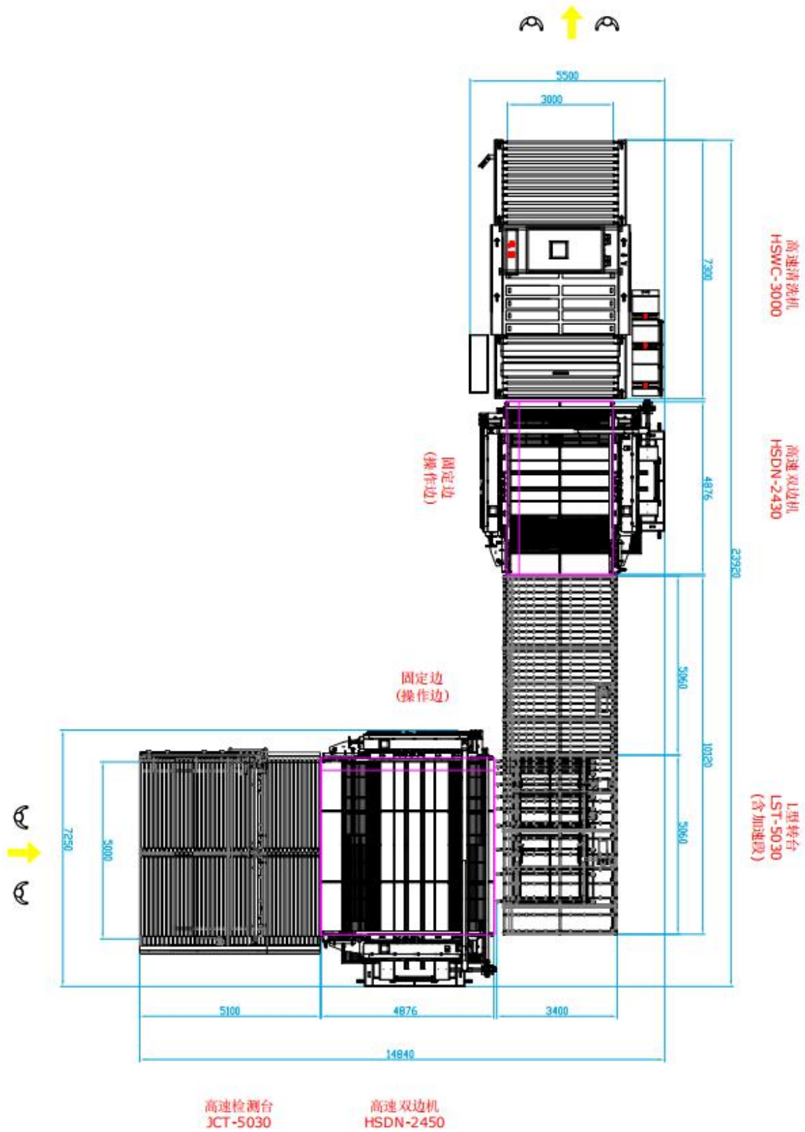
5.0mx3.0mJCT&HSDN24&LST&HSDN24&HSW Sketch Map
