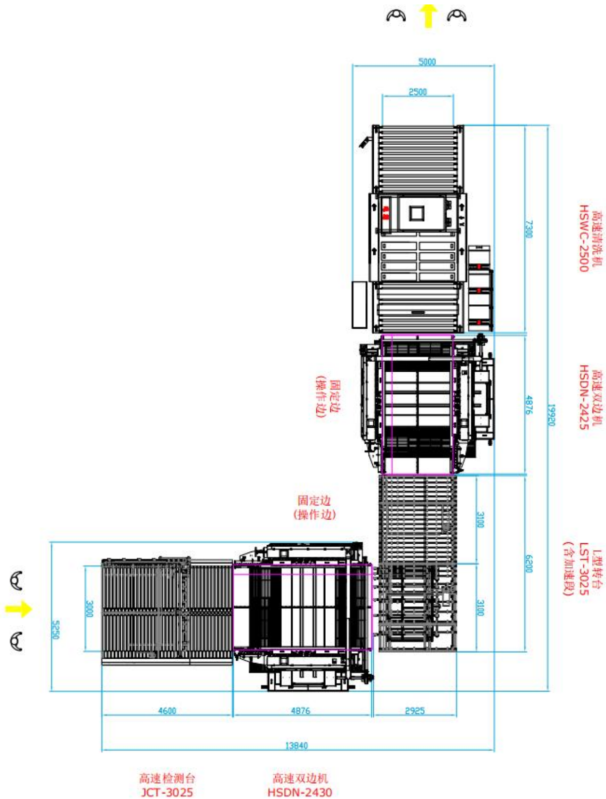
3.0mx2.5mJCT&HSDN24&LST&HSDN24&HSW Sketch Map
