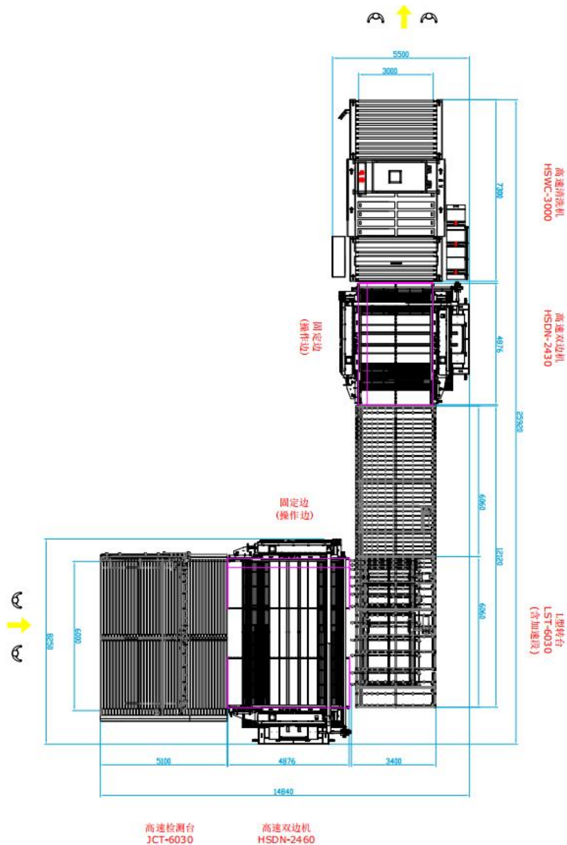
6.0mx3.0mJCT&HSDN24&LST&HSDN24&HSW Sketch Map
