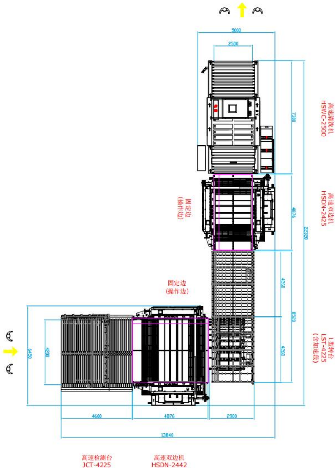
4.2mx2.5mJCT&HSDN24&LST&HSDN24&HSW Sketch Map
